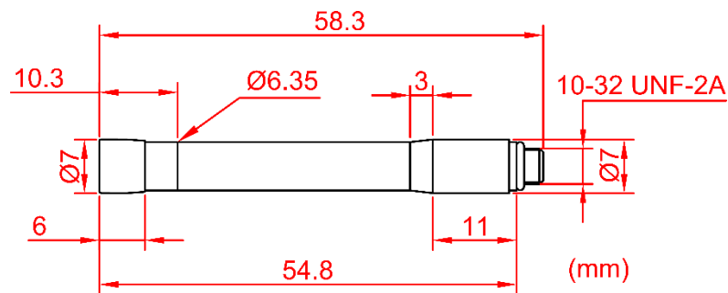
MPA401 with MA411B
