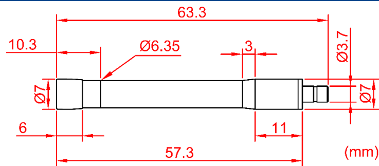
MPA401 with MA411A
