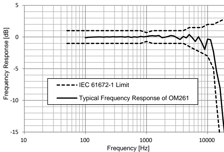
Typical 90° incidence free-field frequency response of OM261
