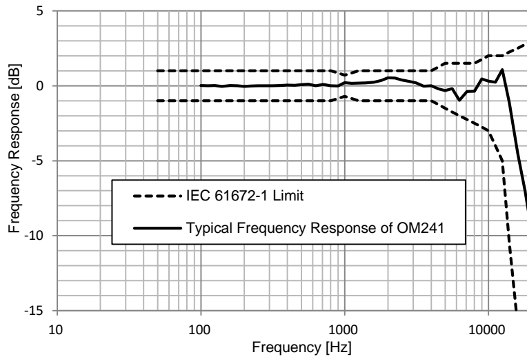
Typical 0° incidence free-field frequency response of OM241
